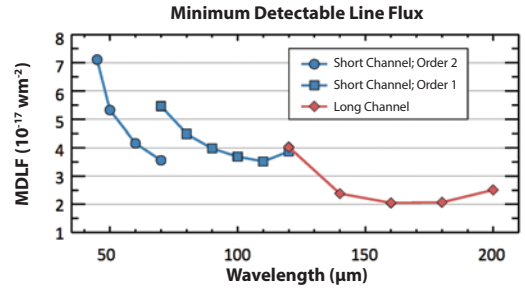
Predicted Sensitivity for SNR = 4 in 900 s
